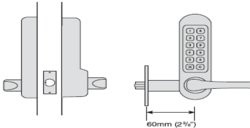
CL510/CL515 with tubular latchbolt
