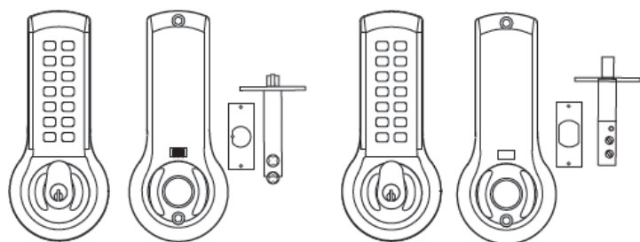
Mortise latch
